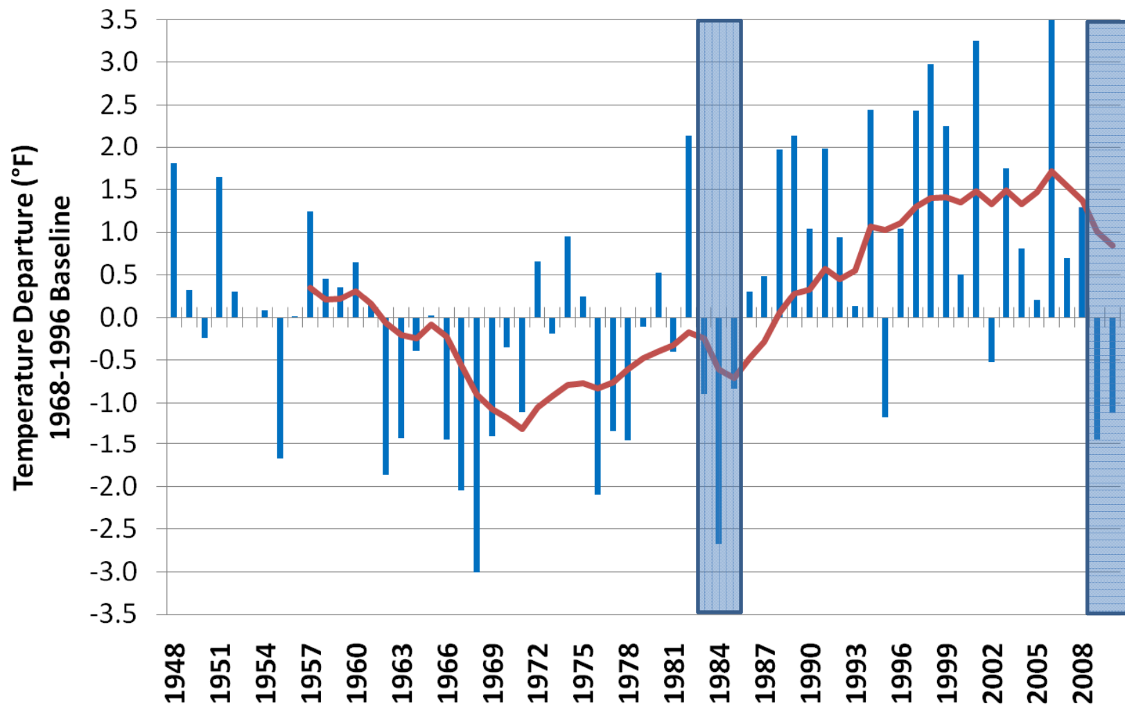
Northern Hemisphere Energy Regions December-February Temperature Departures
