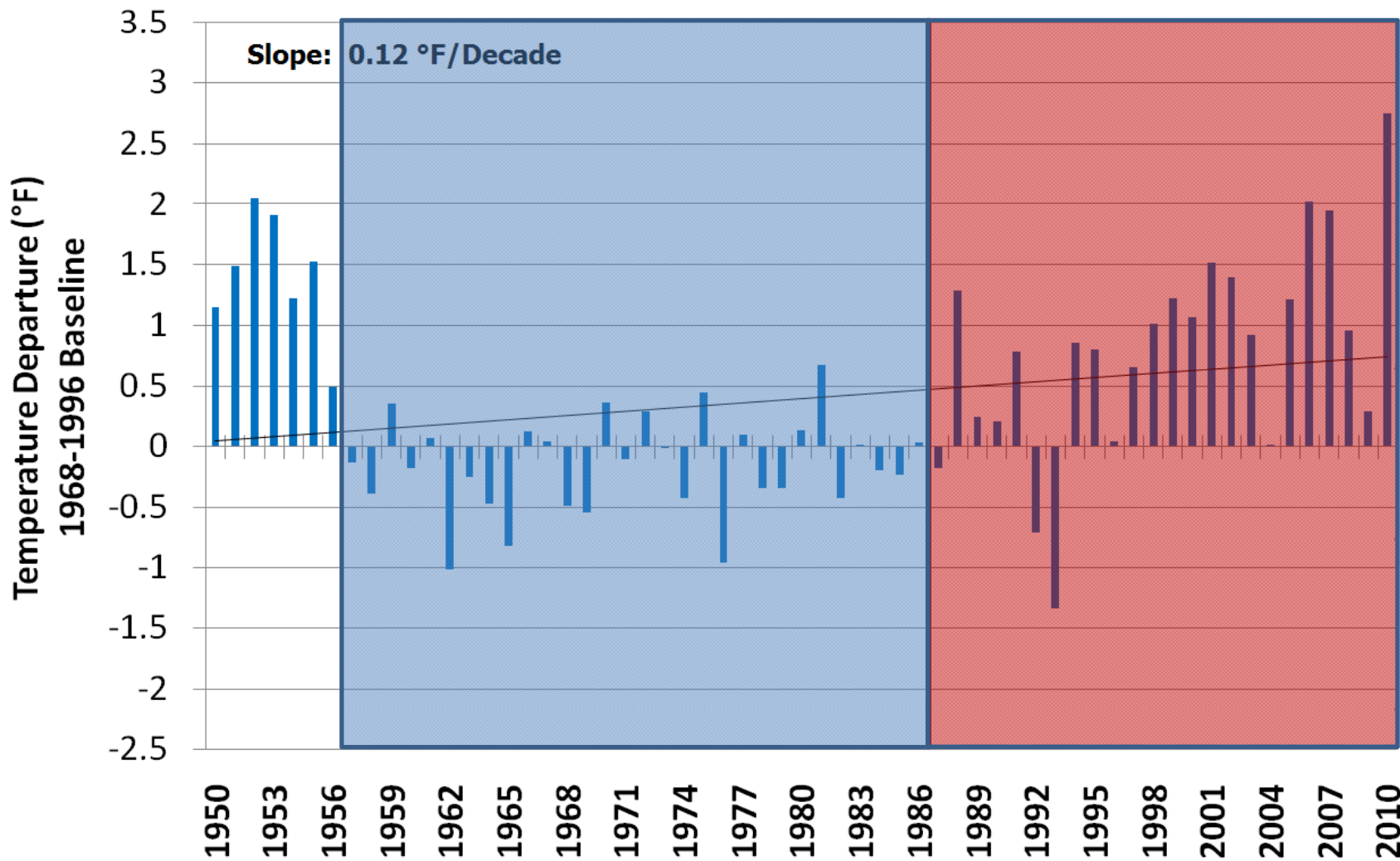
Northern Hemisphere Energy Regions June-August Temperature Departures
