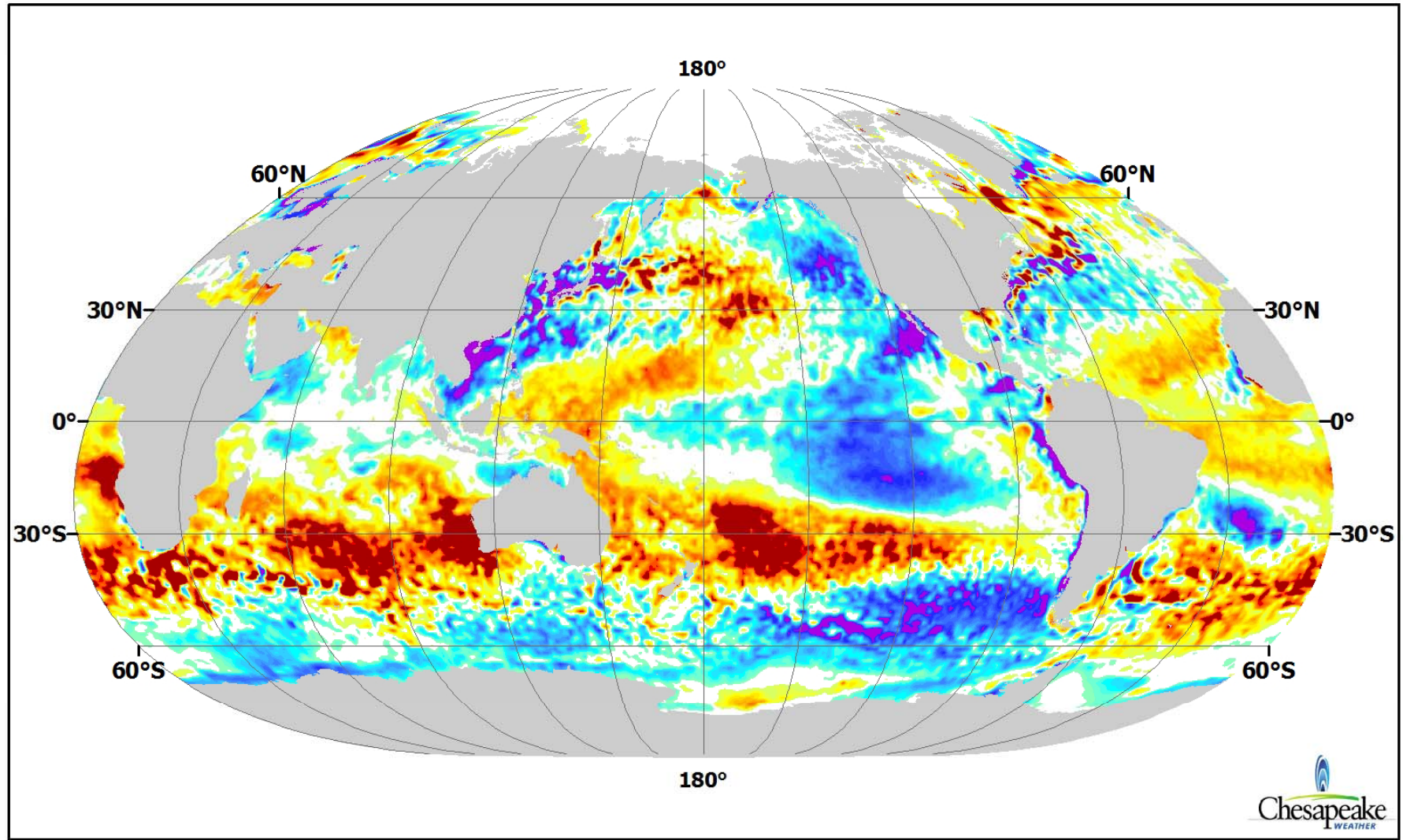
Temp Deviation from Normal (°C)
